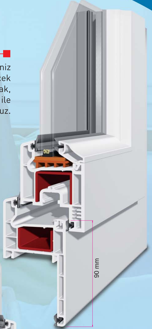
PK60-9 Pervazlı Kasa Cased Frame
